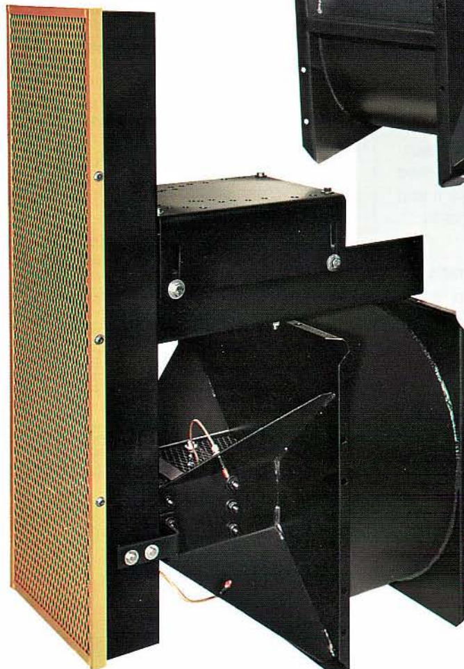
Typical "packaged" SQB fan factory aligned, run tested and ready to install. Includes belt guard and shaft/bearing guard with extended lube lines.
